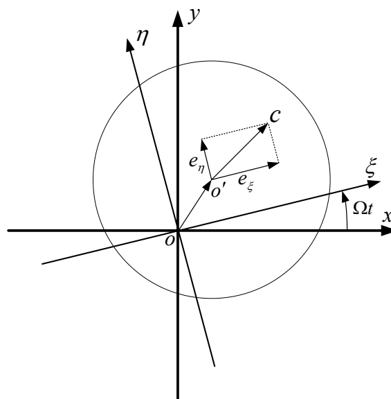
Figure 4. 3. Rotating disk with an imbalance mass
