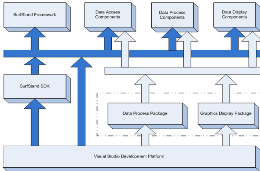
Figure 1: SurfStand System Architecture Diagram
