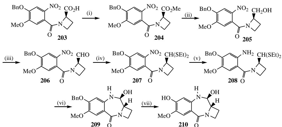
Scheme 1-32 (i) SOCl 2 , MeOH (ii) LiBH 4 , THF, 0°C, r.t. (iii) IBX, DMSO, r.t., 30mins (iv) EtSH, TMSCl, r.t., 12hrs (v) SnCl 2 .2H 2 O, MeOH, reflux, 40mins (vi) HgCl, CaCO 3 , MeCN:H 2 O (4:1), 2.5hrs (vii) 10% Pd/C, cyclohexadiene, EtOH, 45 mins.
