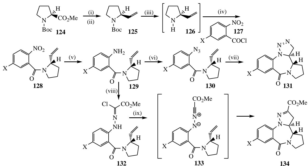
Scheme 1-19 (i) DIBAL-H, dry toluene, N 2 atmosphere, -60°C (ii) Ph 3 PMe + T, t BuOK, dry THF, N 2 atmosphere, 0°C (iii) TFA, N 2 atmosphere, 1hr (iv) K 2 CO 3 , dry toluene, reflux, 4hrs (v) Fe, AcOH, EtOH, reflux, 2hr (vi) NaNO 2 , HCl, Et 2 O, 0°C, 30 mins then NaN 3 , r.t., 40min (vii) CCl 4 , reflux, 5hrs (viii) NaNO 2 /H + then MeCOCHClCO 2 Me (ix) Et 3 N, toluene, reflux.
