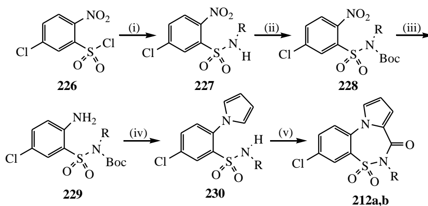
Scheme 1-35 (i) \text{R-NH}_2 (ii) (\text{Boc})_2\text{O} , DMAP (iii) \text{Fe} , \text{AcOH} (iv) 2,5-dimethoxytetrahydrofuran, \text{AcOH} (v) triphosgene \text{R} = \text{H} , Et.
