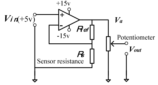
Fig.4 Circuit diagram used with each of the four sensors
