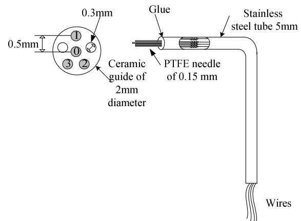
Fig. 1 Schematic of four-sensor probe
