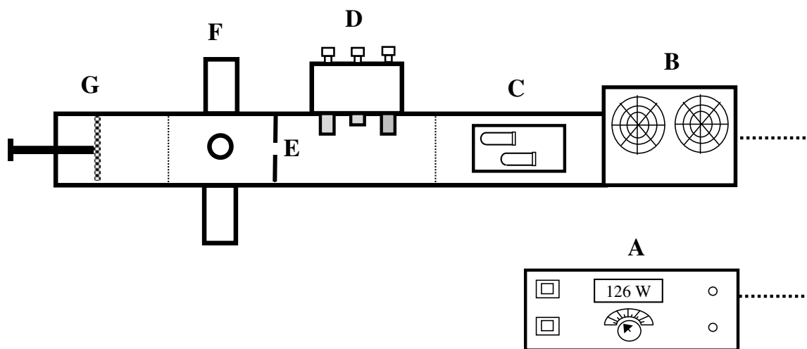
FIG. 1. Schematic diagram of the single-mode microwave system A: 1000 W variable microwave power unit; B: air-cooled generator and launch section; C: water-cooled circulator; D: manual 3-stub unit; E: iris plate; F: 4-port heating section; G: variable short circuit (plunge tuner)
