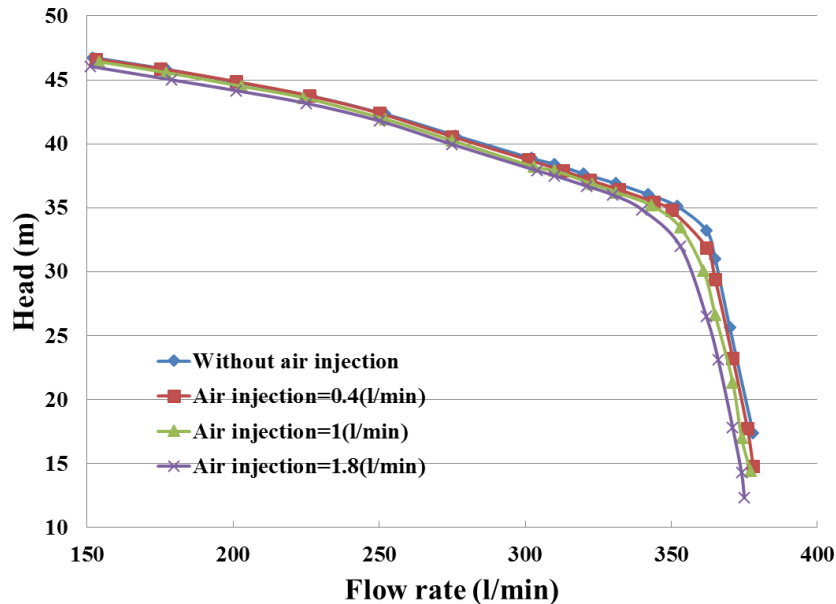
Figure 6-38: Head of the pump with and without air injection under different air injections
