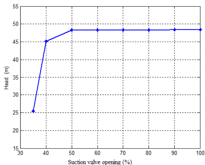
Figure 6-21: The relation between head and different suction valve openings at 103(l/min)
