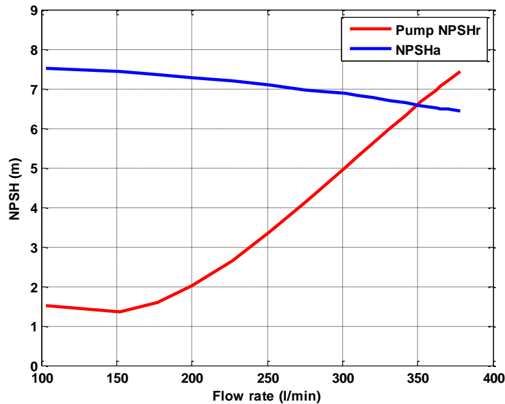
Figure 6-4: The cavitation characteristics of the centrifugal pump under different flow rates
