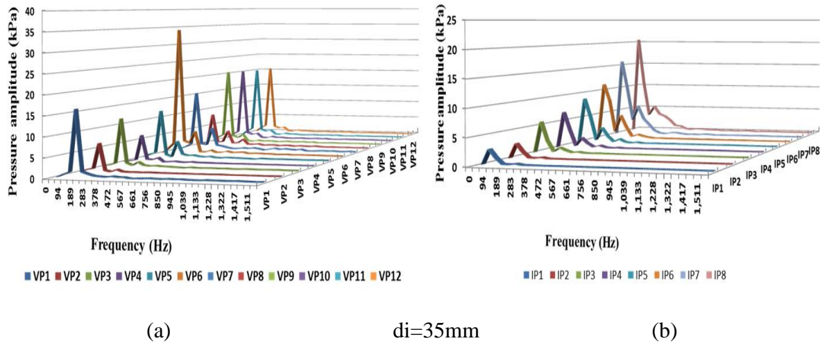
Figure 5-54: (a) Frequency spectra around the volute and (b) At the impeller under different inlet impeller diameters
