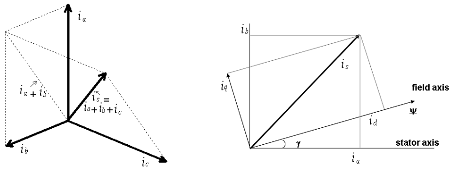
Figure 3.19 The principle of FOC control [87]
