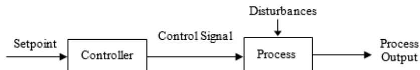
Figure 3.1 Input-output configuration of an open loop control system, redrawn [72].
