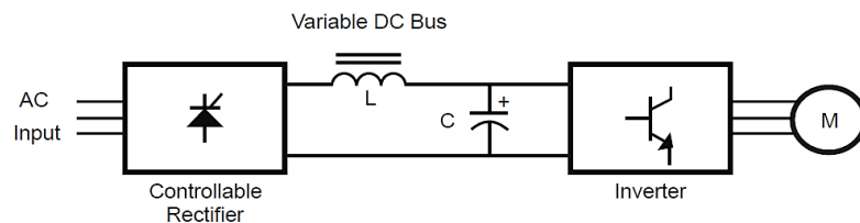
Figure 3.17 Block diagram of a typical VVI drive [8].
