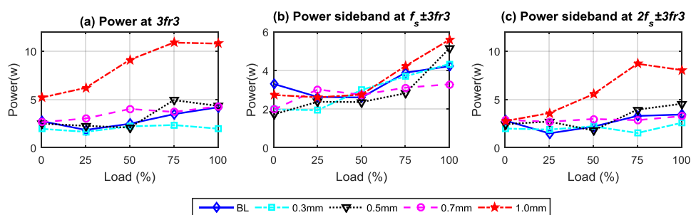
Figure 7.21 Power at f_{r3} , and corresponding sidebands under different operating conditions
