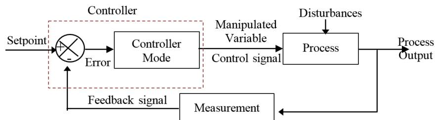
Figure 3.2 Block diagram of a closed loop control system, adapted from [71].
