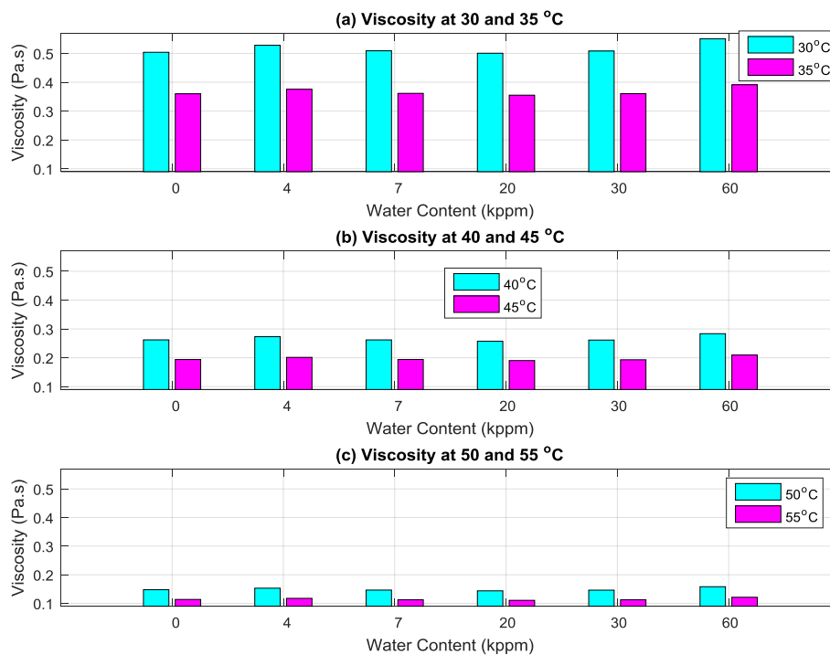
Figure 8.2 Viscosity with different water contents at different temperature values
