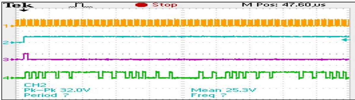
Figure 8.28 The DiPPM Deoder Waveform Single Codeword Output
