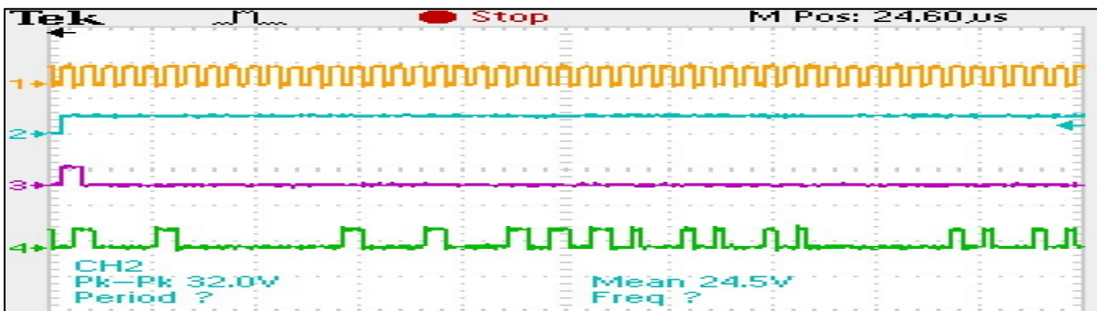
Figure 8.24 The DiPPM Coder Waveform Single Codeword Output
