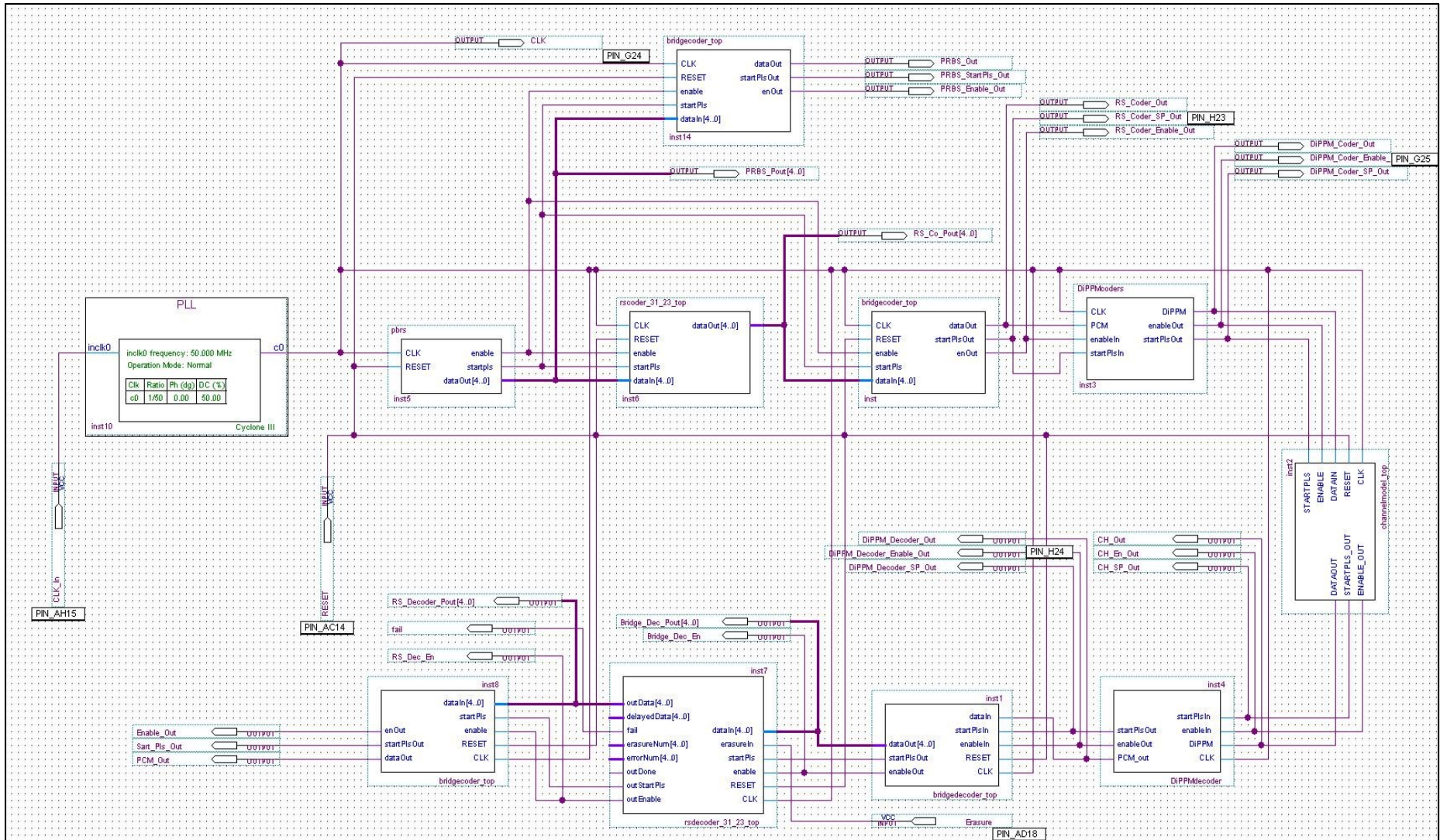
Figure 8.14 The DiPPM with (31,23) RS Code System
