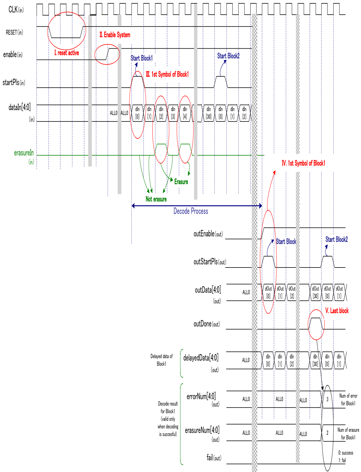
Figure 6.27 RS(31,23) decoder timing chart
