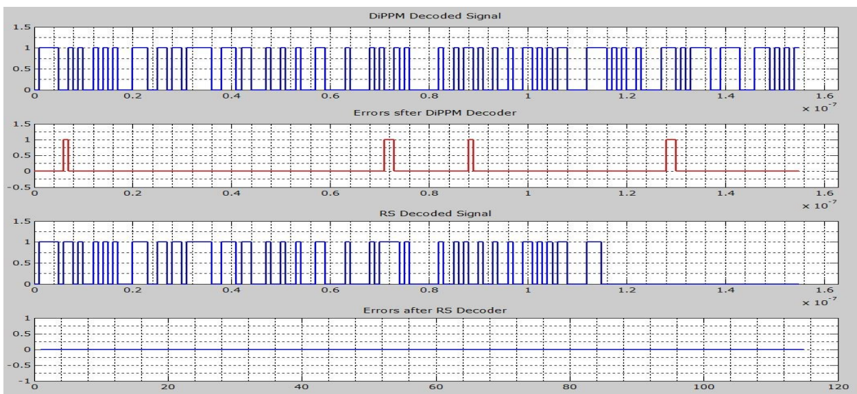
Figure 5.6 DiPPM with RS code Rx output waveform
