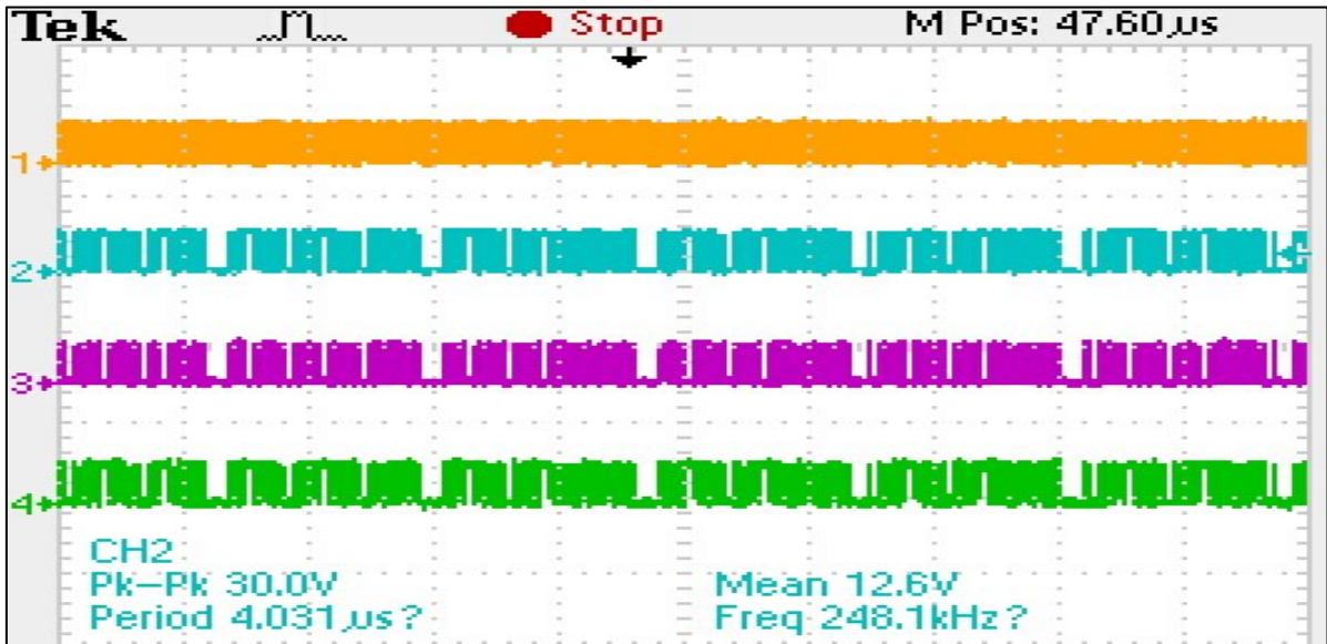
Figure 8.29 Comparison between RS Coder (blue), DiPPM Coder (purple), and DiPPM Decoder (green) Multi codewords output waveforms
