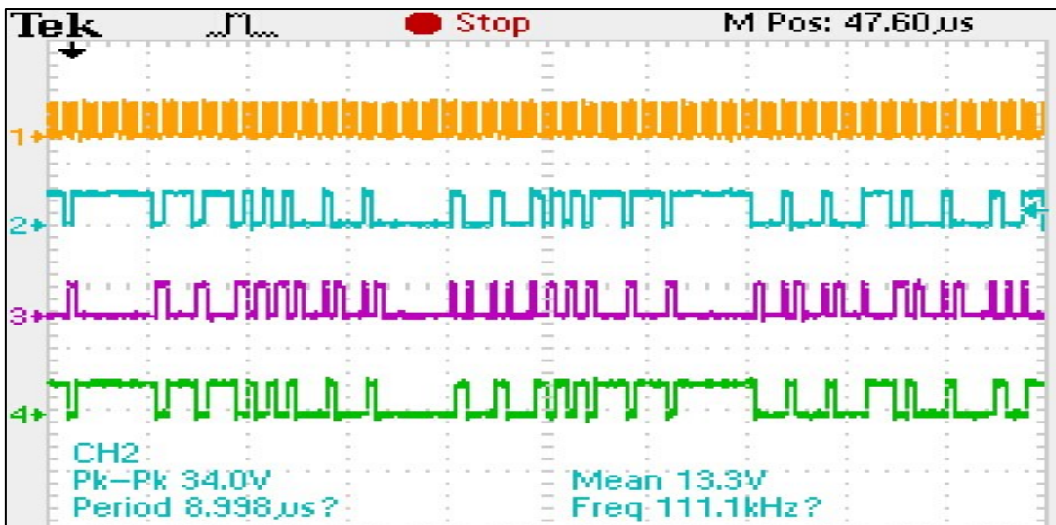
Figure 8.30 Comparison between RS Coder (blue), DiPPM Coder (purple), and DiPPM Decoder (green) Single codeword output waveforms
