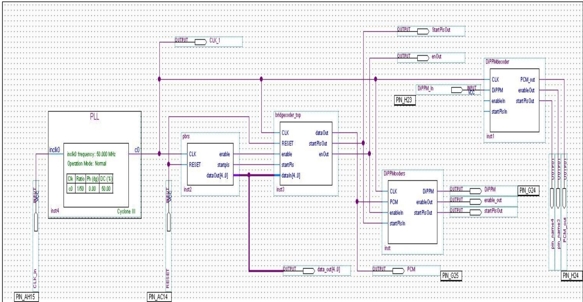
Figure 8.12 DiPPM system design on Altera Quartus II
