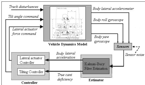
Figure 6: NDAC configuration
