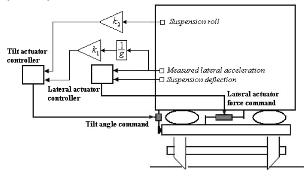
Figure 5: CDAC configuration
