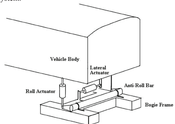
Figure 1: The integration of roll and lateral actuators
