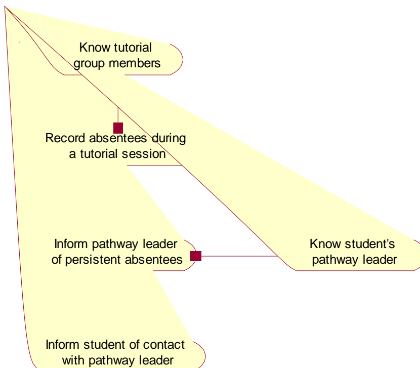
Figure 4. Activity Diagram for Attendance Monitoring
