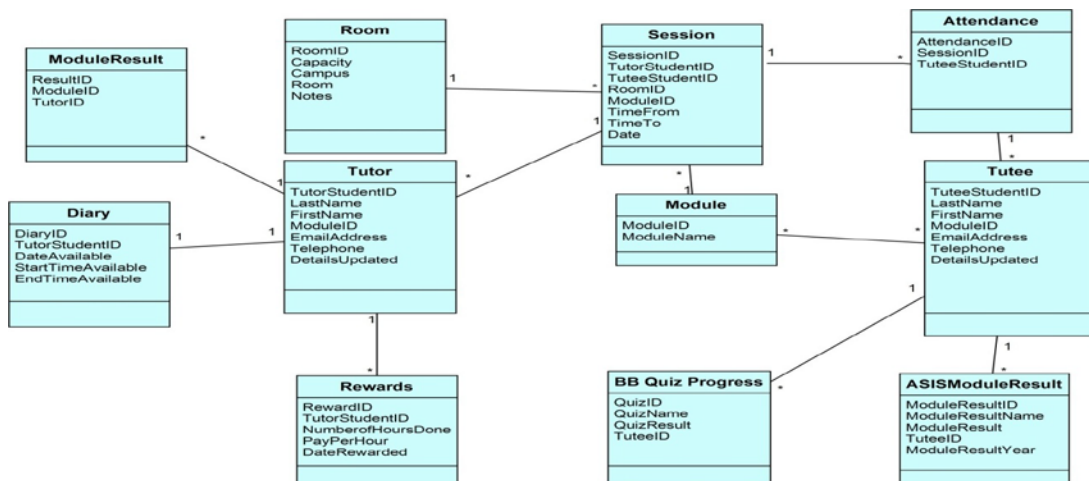
Figure 10: Class diagram
