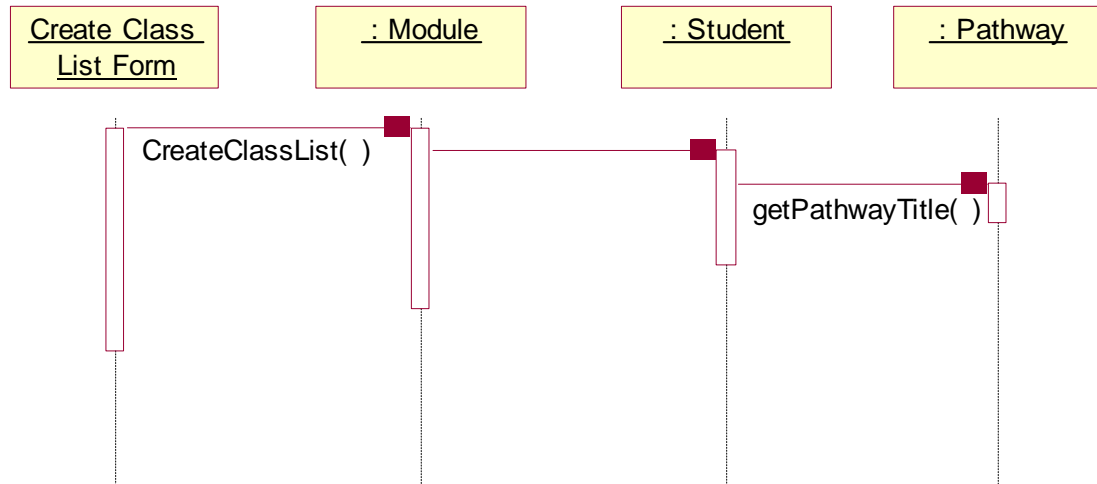
Figure 7. A sequence Diagram.
