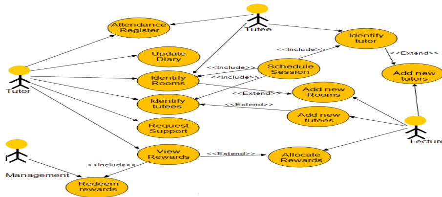
Figure 9: Peer-Tutoring System Use Case Diagram
