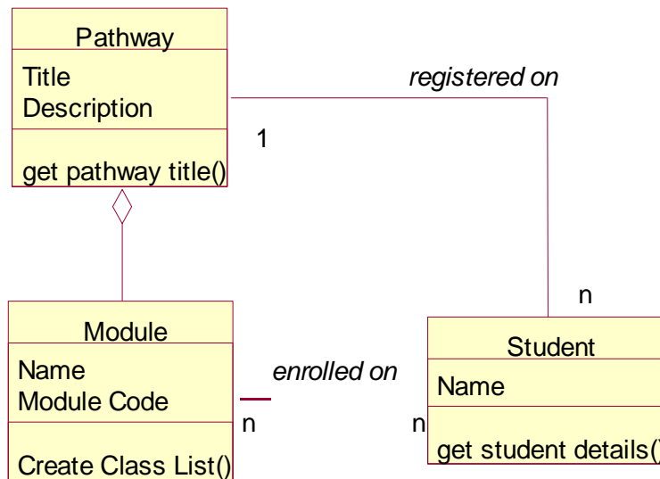
Figure 8: A Domain Model
