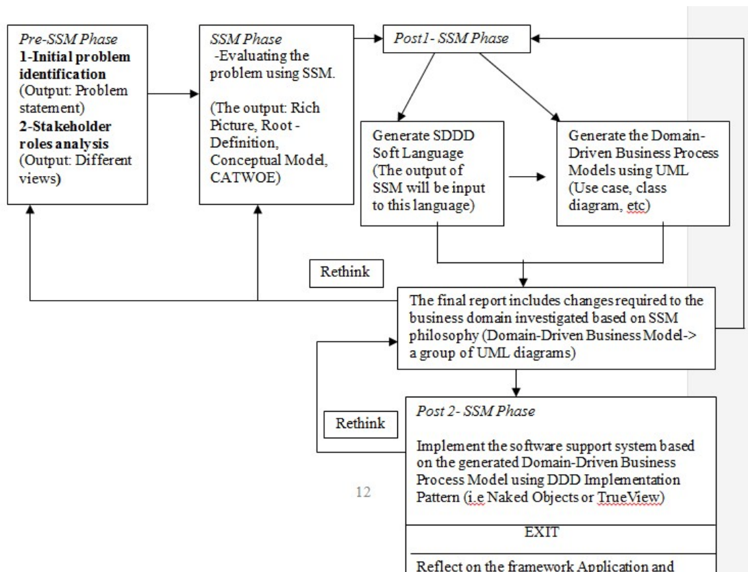
Figure 1 –The SDDD Framework
