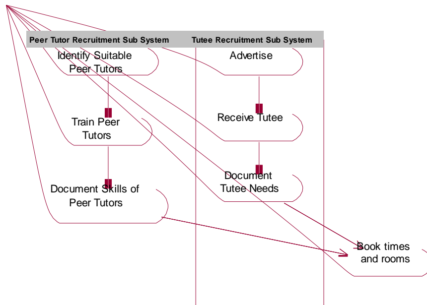
Figure3: Activity diagram of Peer Tutor and Tutee recruitment subsystems
