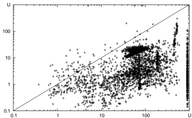
Figure 2: CPU time (log. scale) of LPG.sd versus LPG.d for the problems in benchmark set MS. The x-axis shows runtime of LPG.d and the y-axis runtime of the specific LPG.sd solvers, measured in CPU seconds; U indicates runs that timed out with the given runtime cutoff.
